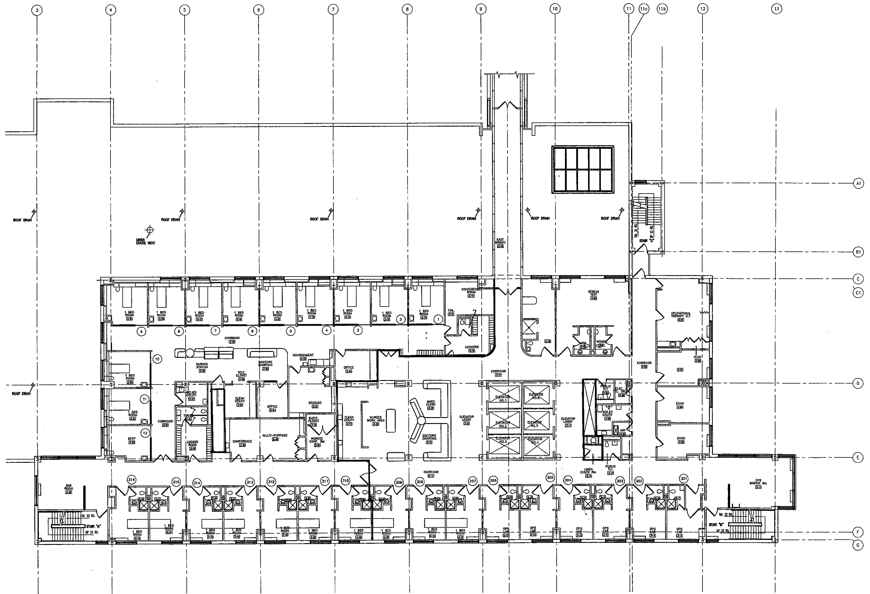
A THIRD FLOOR PLAN A-B SCALE: 1/8" = 1'-0"
